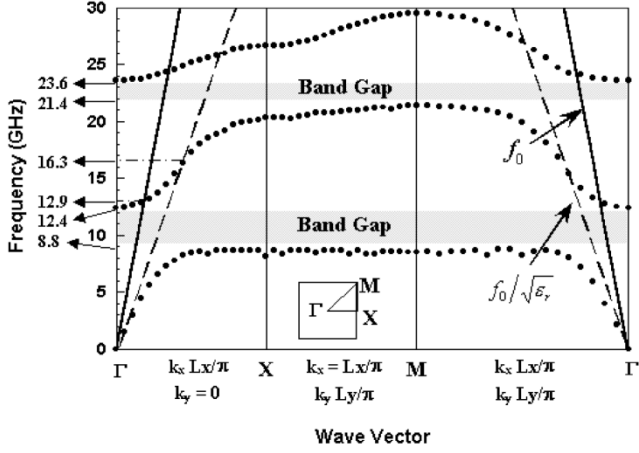
Fig. 2. Dispersion diagram of the MS using the unit cell of Fig. 1(b). Lx and Ly denote the lengths of the PBG unit cell in the x and y directions, respectively. k_x and k_y denote the wave numbers of the PBG unit cell in the x and y directions, respectively.
