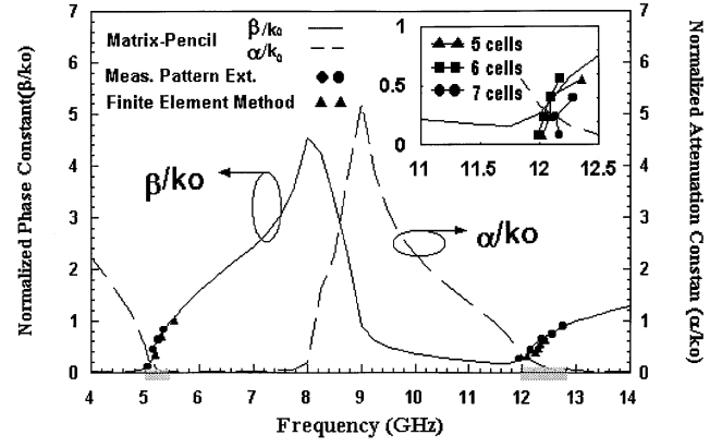
Fig. 7. Normalized phase constant \beta/k_0 and normalized attenuation constant \alpha/k_0 of the leaky mode of the EME microstrip propagating in the forward direction.
